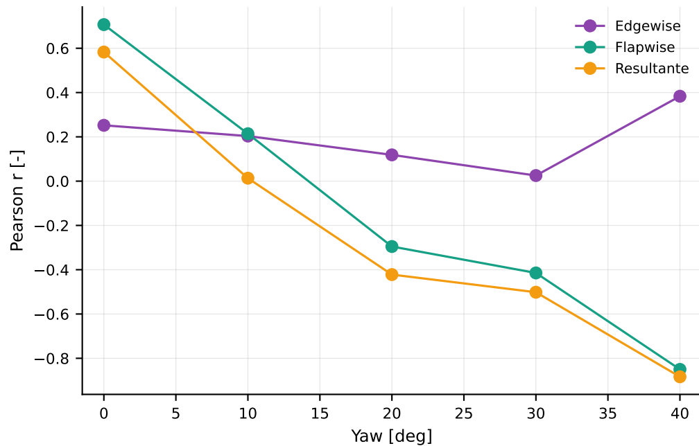
(a) Correlation with torque
