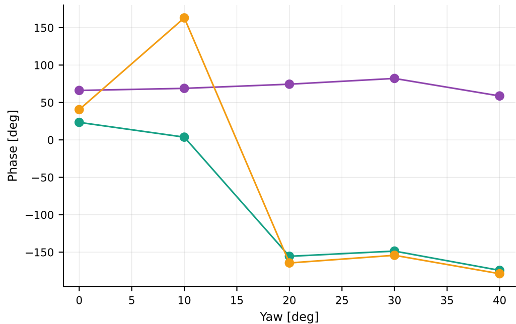
(b) Torque phase relative to deformation
