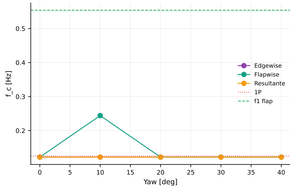
(a) Dominant coupling frequency
