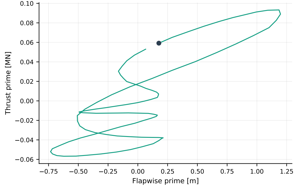
(b) Thrust prime vs flapwise prime
