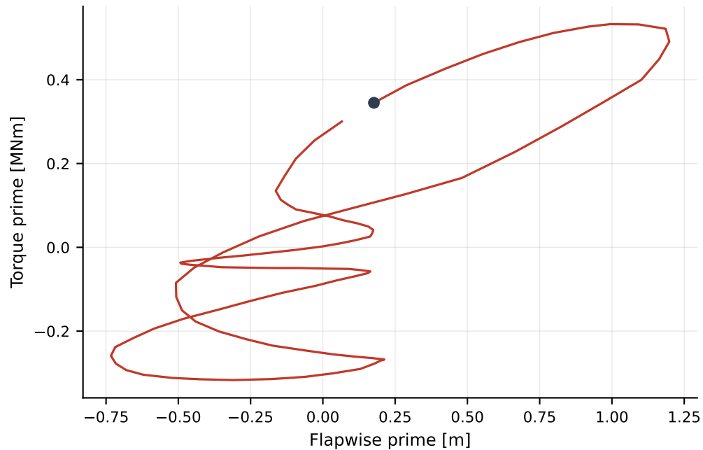
(a) Torque prime vs flapwise prime
