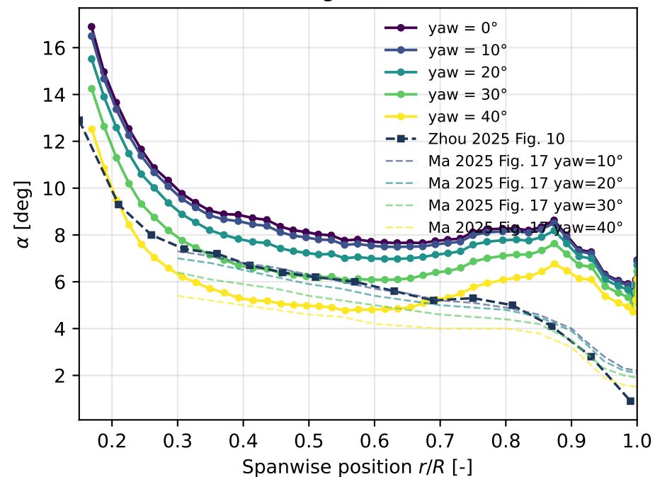
(a) Angle of attack
