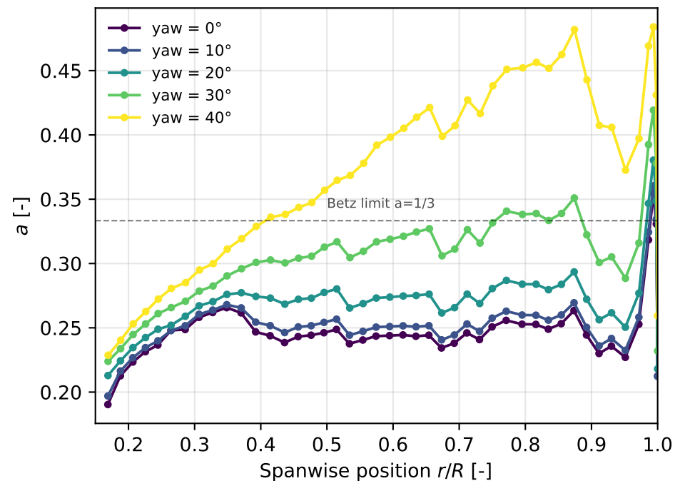
(b) Axial induction factor
