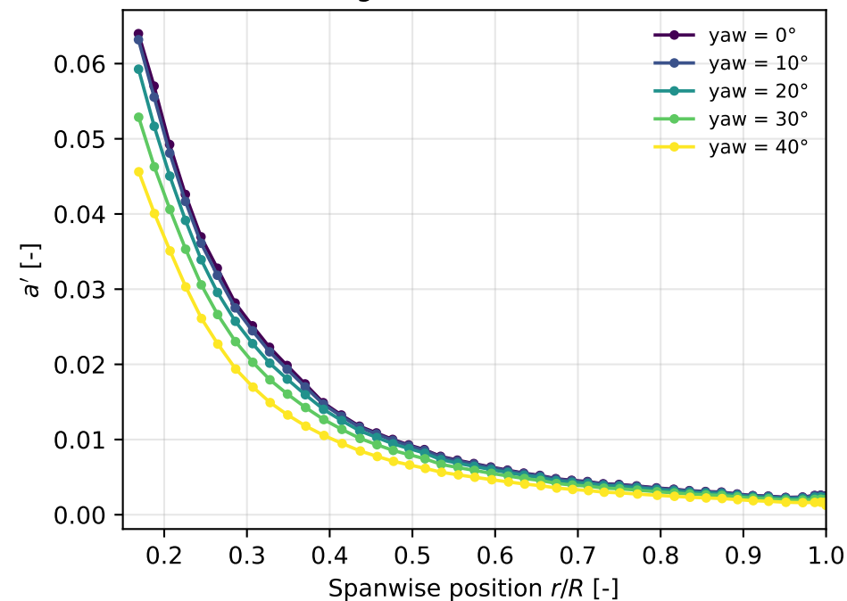
(c) Tangential induction factor
