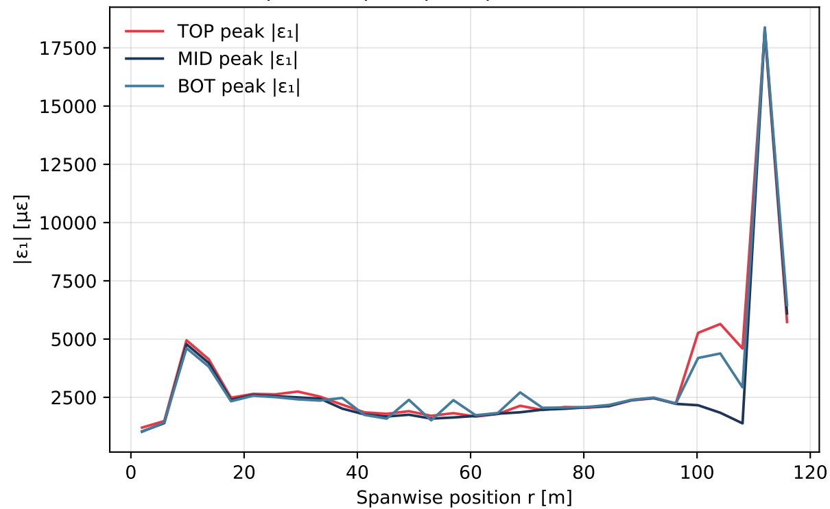
(c) Spanwise peak principal strain (30 bands)
