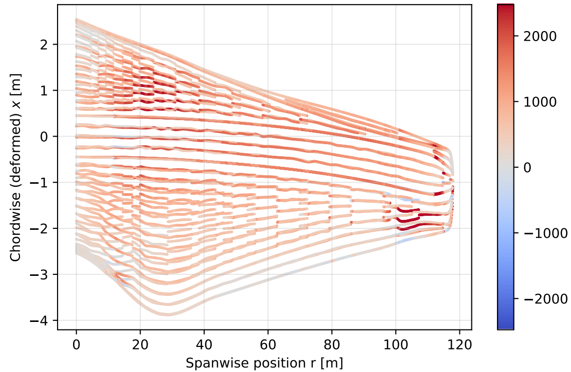
(c) Spanwise peak principal strain (30 bands)
