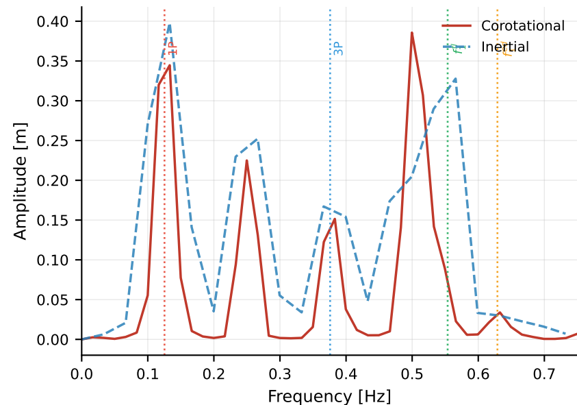
(a) Flapwise tip deflection
