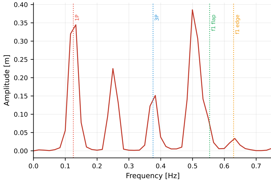
(a) Flapwise tip FFT
