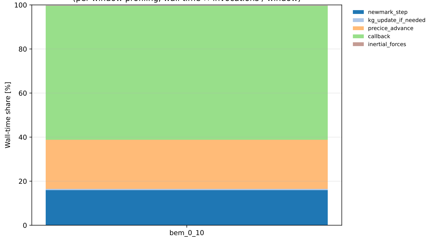
AeroElast computational cost breakdown by phase (per-window profiling, wall time \times invocations / window)
