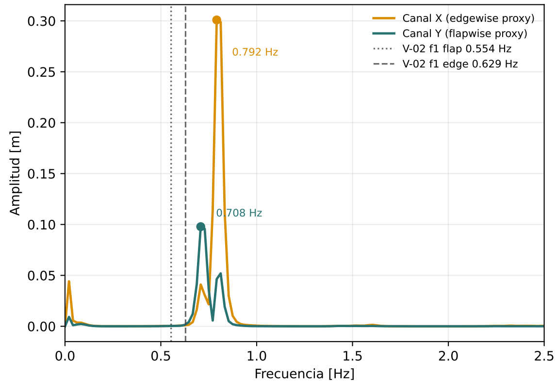
FFT one-sided, Hann, Delta f = 0.0208 Hz
