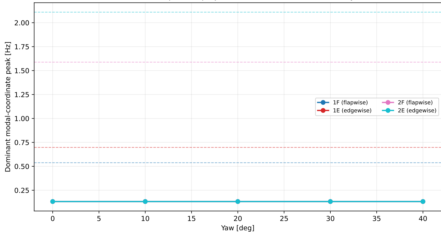
Dominant FFT peak of projected modal coordinates across yaw
