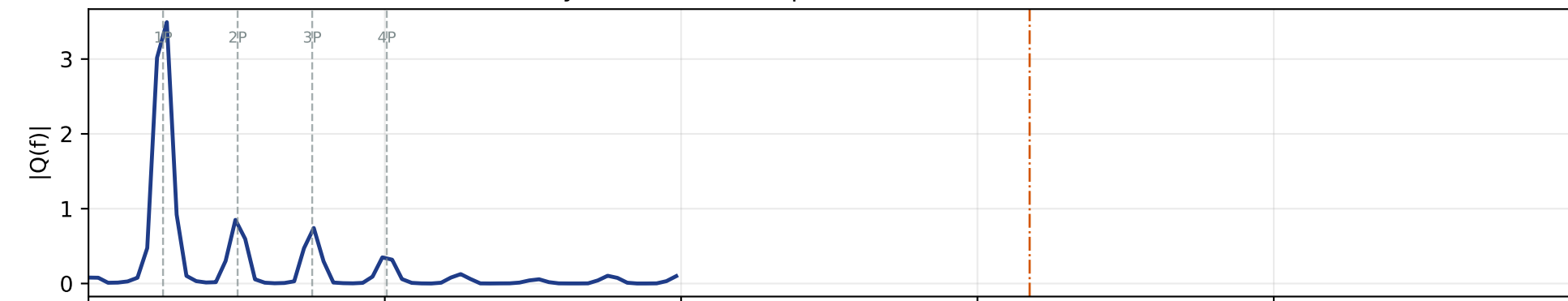
yaw=0° — 2E (edgewise) basis=2.110 Hz
