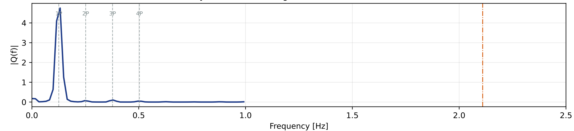
yaw=0° — 2E (edgewise) basis=2.110 Hz
