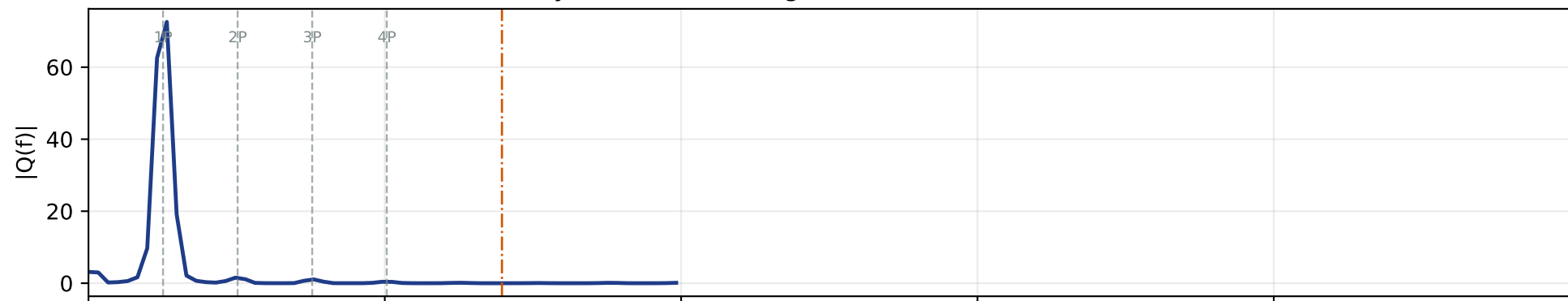
yaw=0° — 2F (flapwise) basis=1.588 Hz
