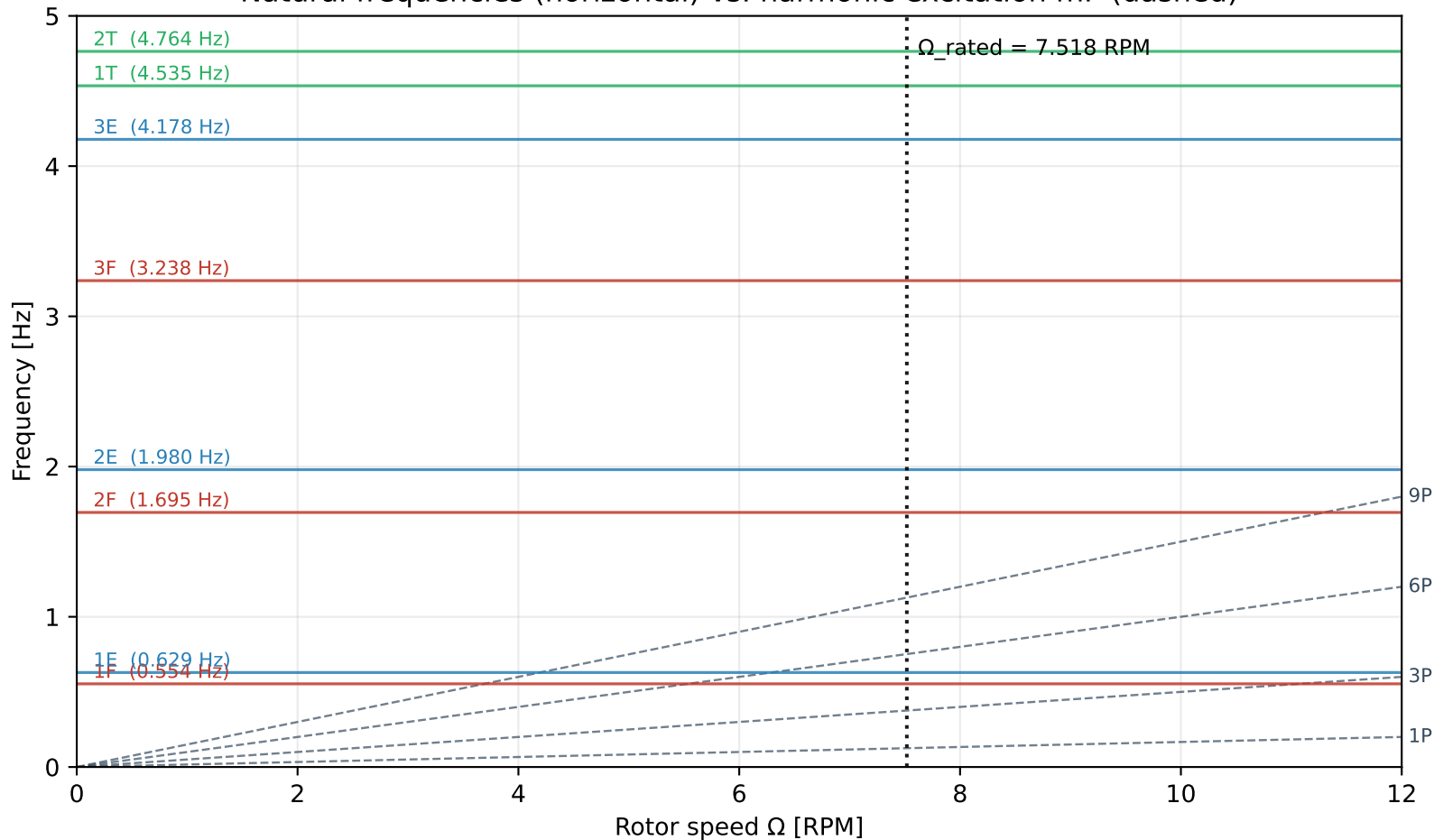
Campbell diagram — IEA 15 MW blade (static, no centrifugal stiffening) Natural frequencies (horizontal) vs. harmonic excitation mP (dashed)
