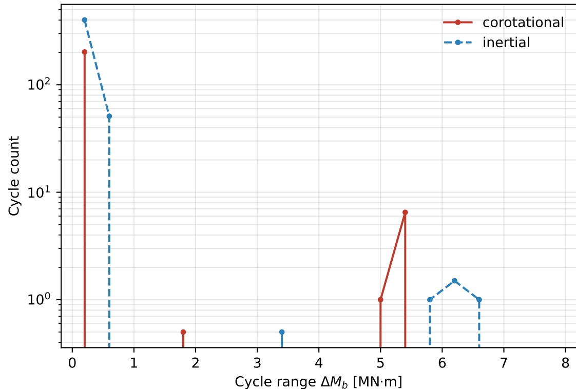
Rainflow cycle histogram — yaw=0°
