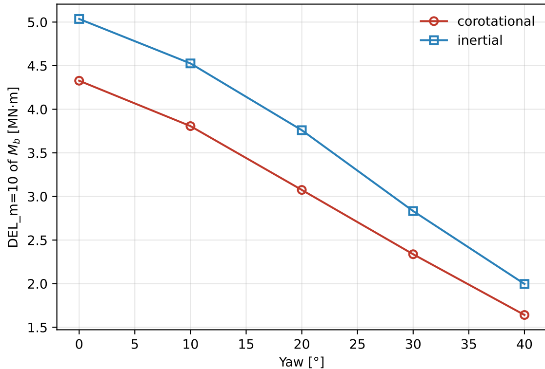
Damage Equivalent Load — M_b root, Wöhler slope m=10
