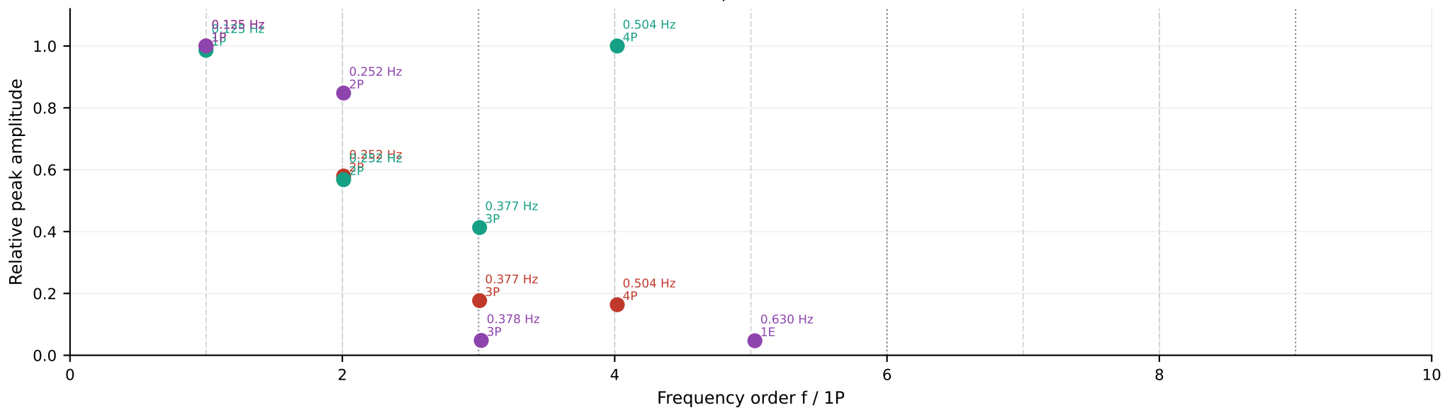
(b) Peak locations as P-order; multiples of 3 survive ideal 3-blade summation
