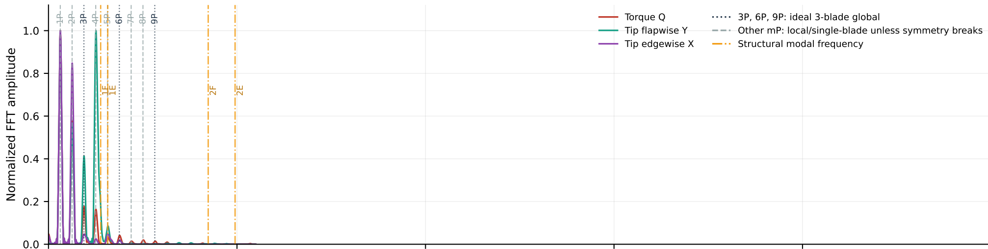
(b) Peak locations as P-order; multiples of 3 survive ideal 3-blade summation
