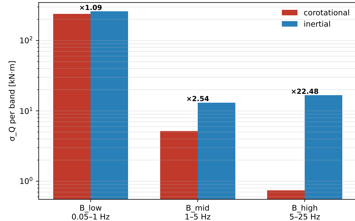
Torque sub-band variance — yaw=0°
