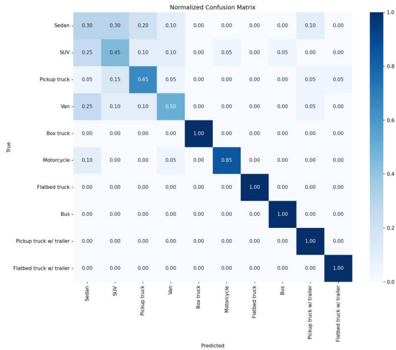
Figure 3 — Normalized confusion matrix after 1 epoch
