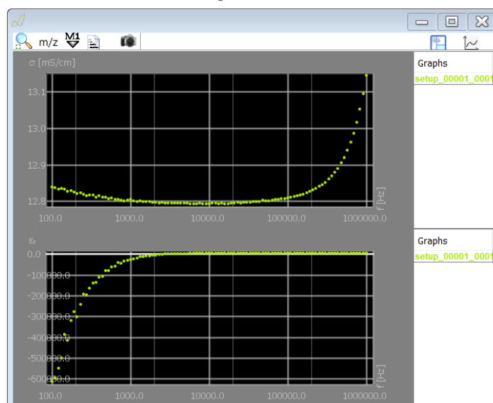
Figure 13: conductivity plot
