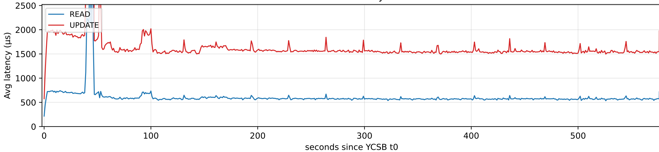
YCSB latency
