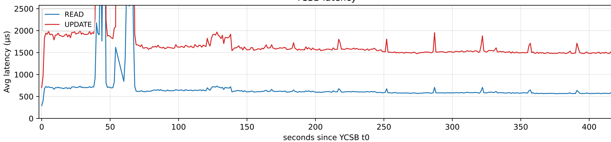
YCSB latency
