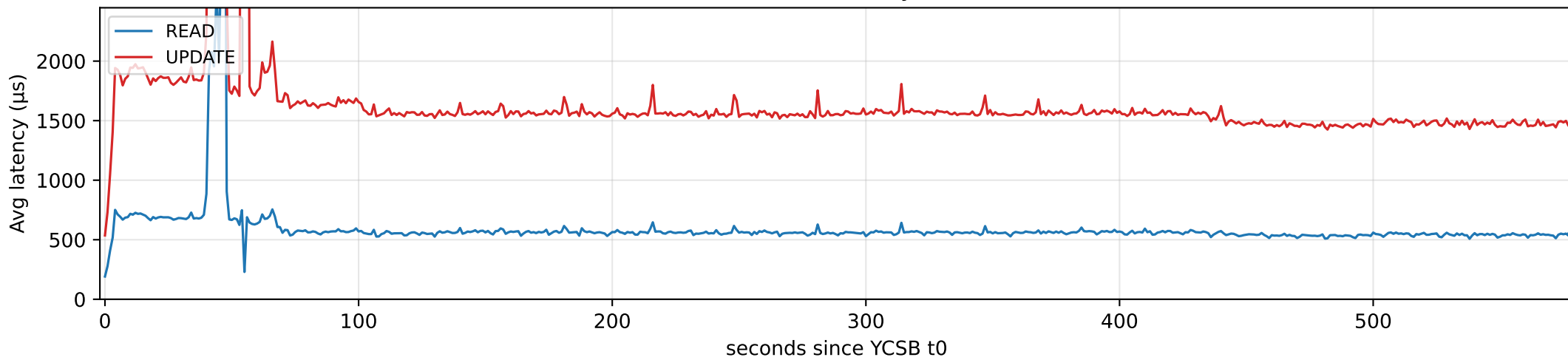
YCSB latency
