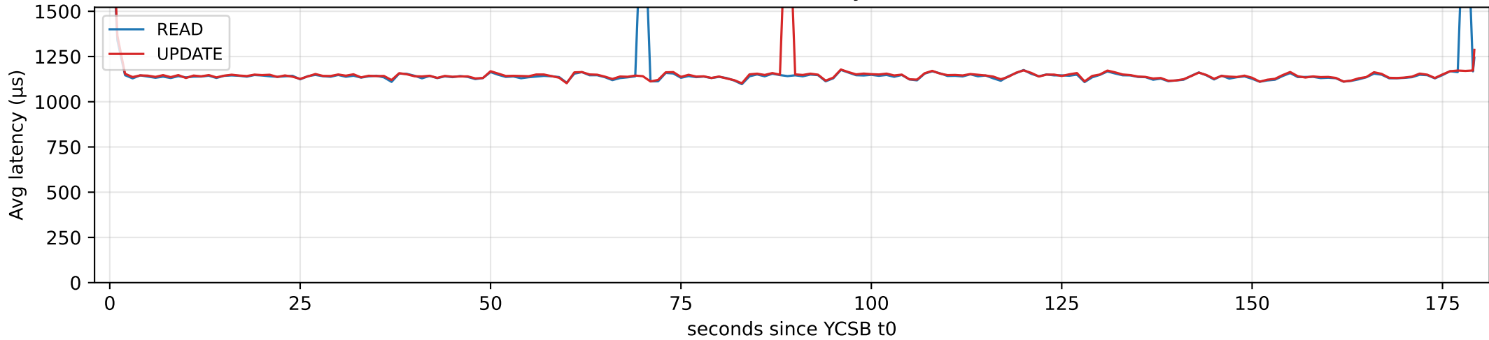
YCSB latency
