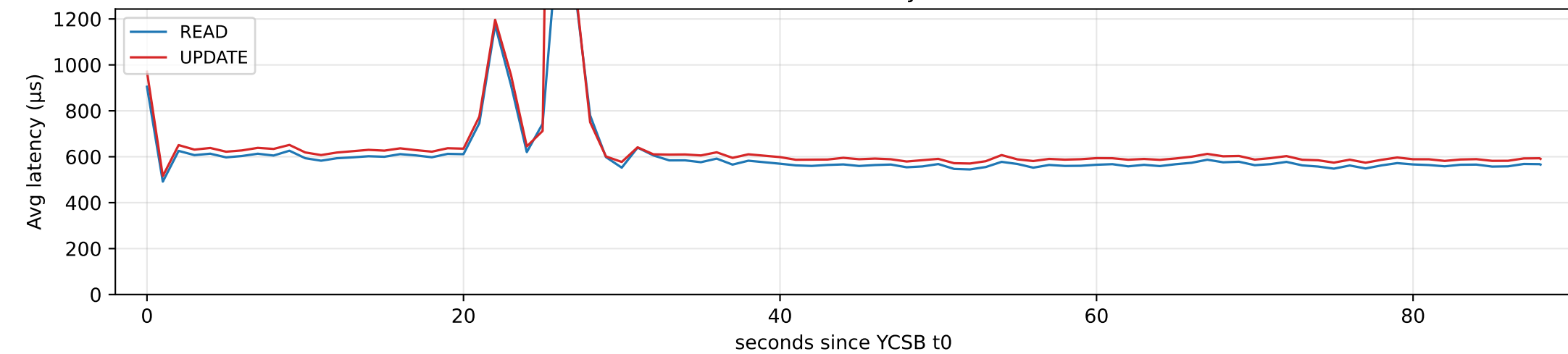
YCSB latency
