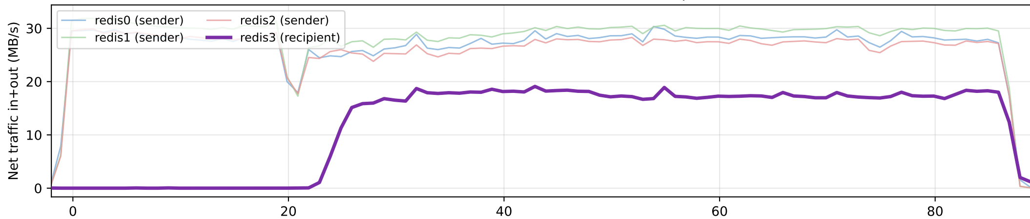
YCSB throughput
