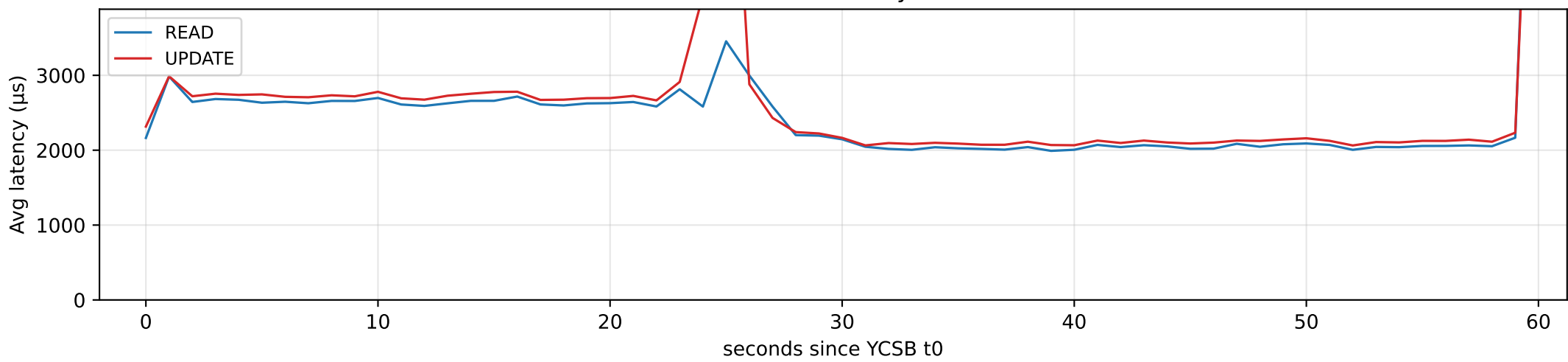
YCSB latency
