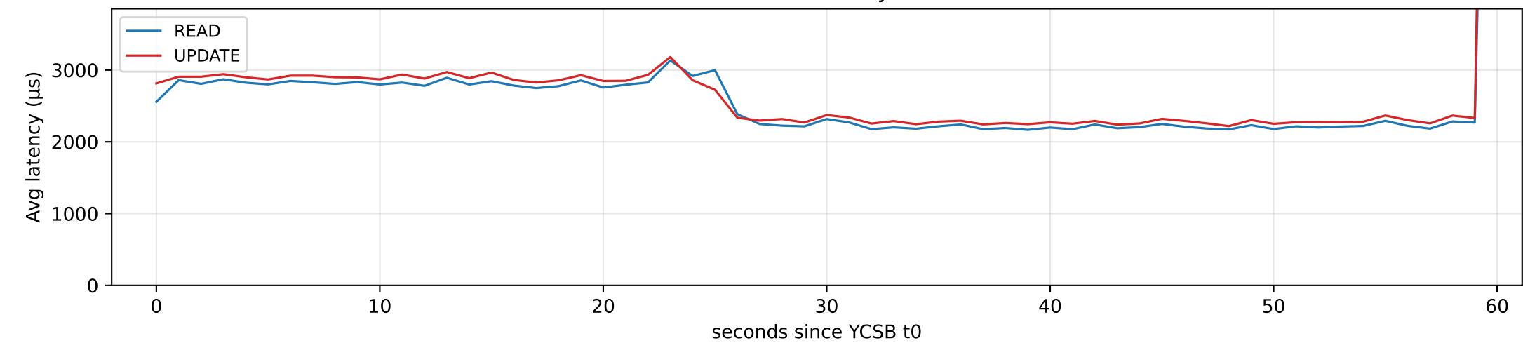
YCSB latency
