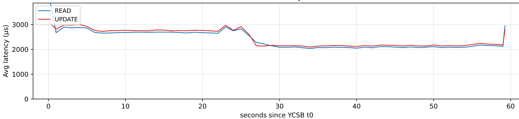
YCSB latency
