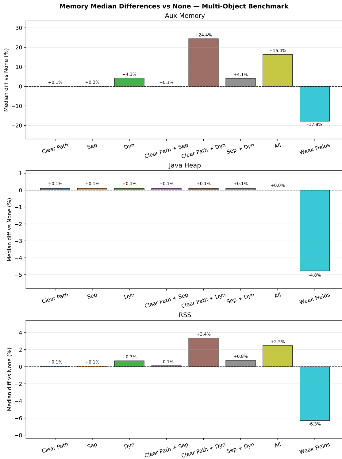
Figure 4.12. Median percentage difference in per-run maximum memory usage relative to the none baseline, multi-object benchmark . Lower is better. Top to bottom: auxiliary GC memory, Java heap, total process RSS.
