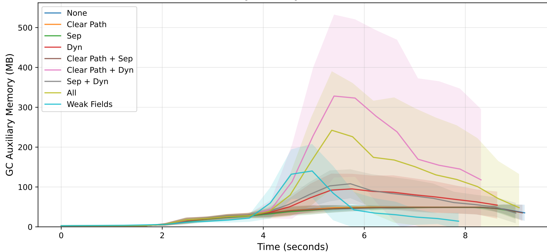
GC Auxiliary Memory (Mean \pm Std Dev)
