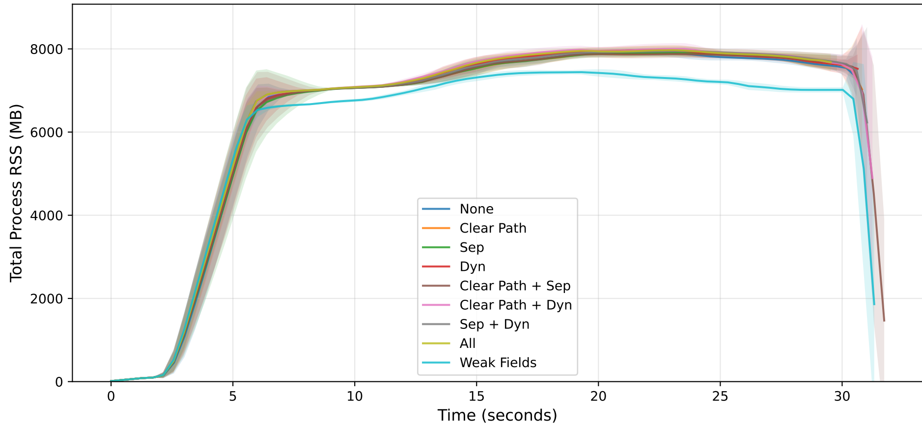
Total Process Memory (Mean \pm Std Dev)
