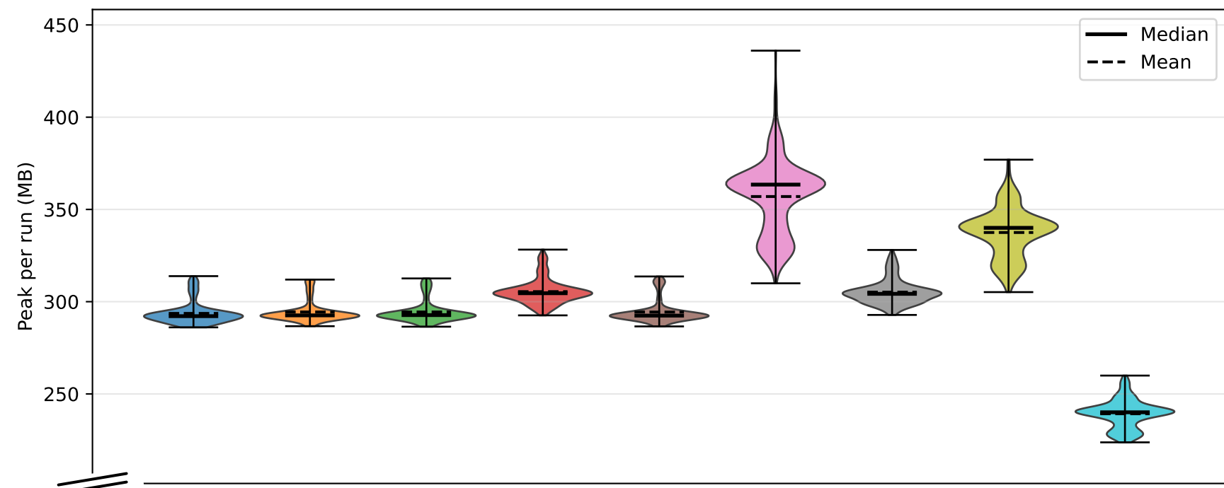
Auxiliary GCr Memory — Multi-Object Benchmark
