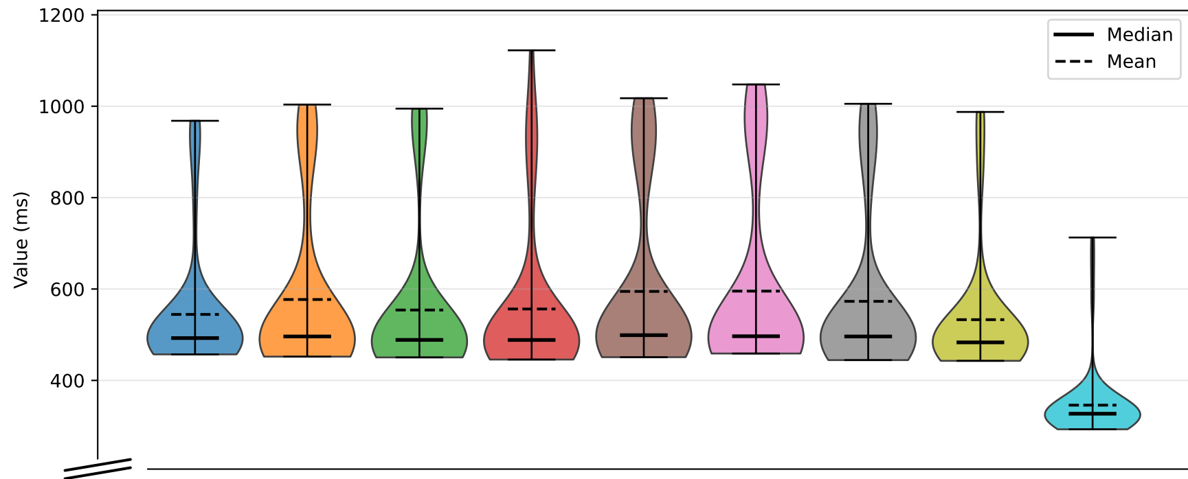
Young Generation: Young Generation (Promote All) — Single-Object Benchmark
