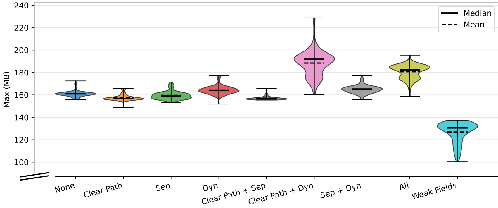
Java Heap
