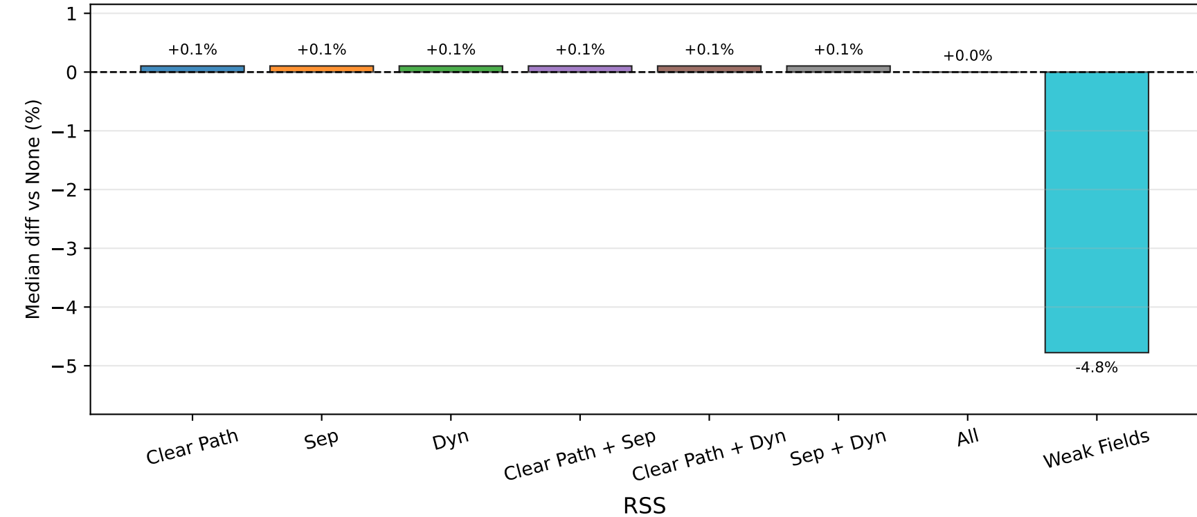
Java Heap
