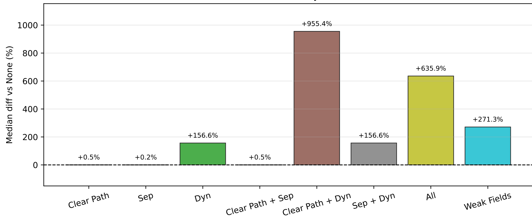
Java Heap
