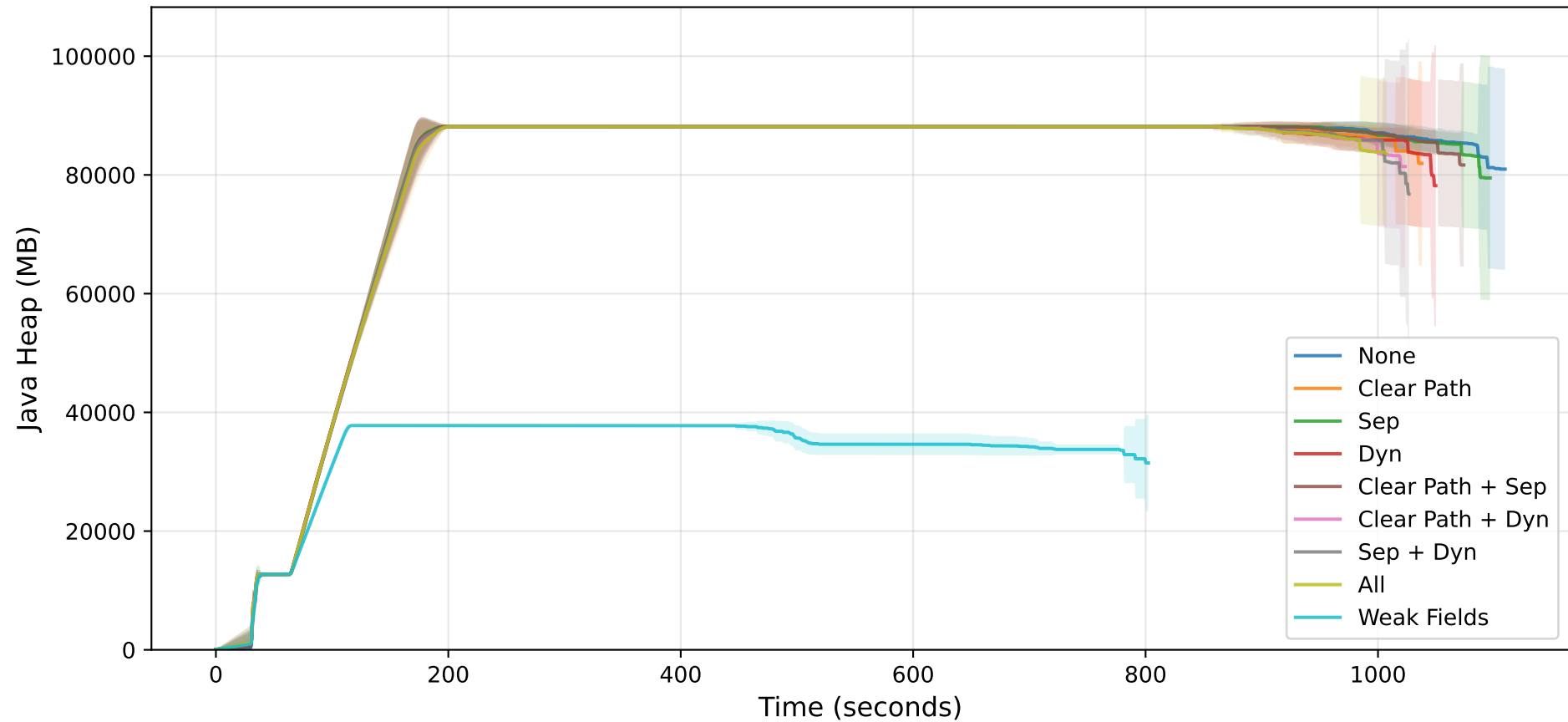
Java Heap Usage (Mean \pm Std Dev)
