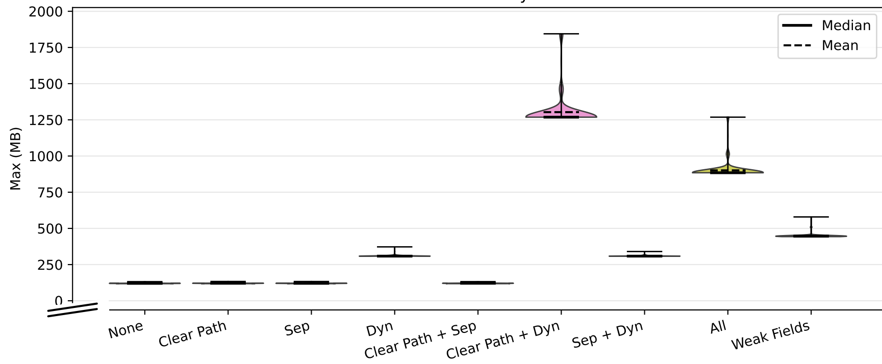
Java Heap
