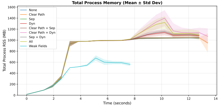
(a) Total Process RSS
