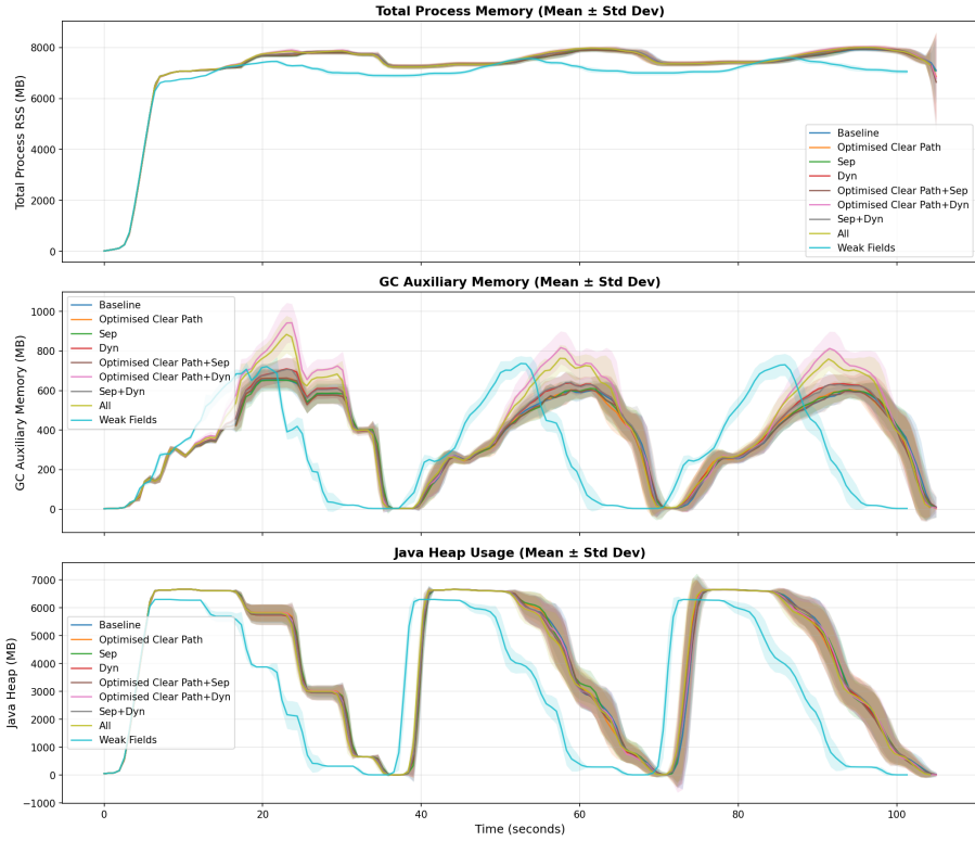
Figure 4.4. Continuous memory trace for the multi-object benchmark.
