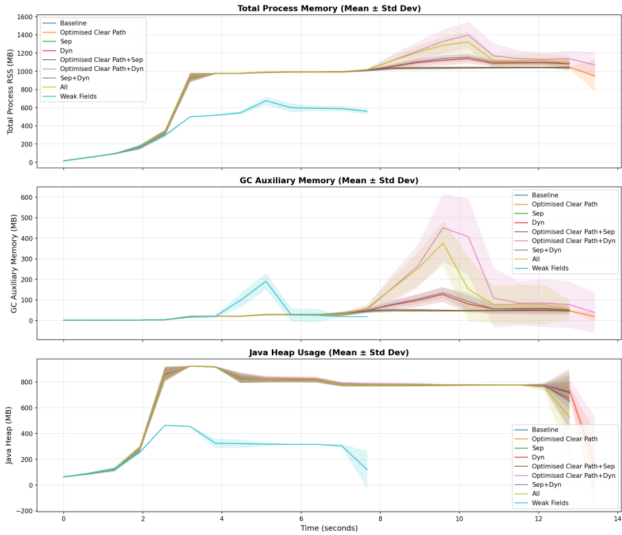
Figure 4.3. Continuous memory trace for the single-object benchmark.
