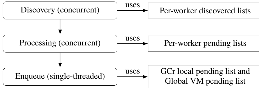
Figure 2.2. ZGC reference-processing pipeline and data flow from discovery to Java-level enqueue handling.
