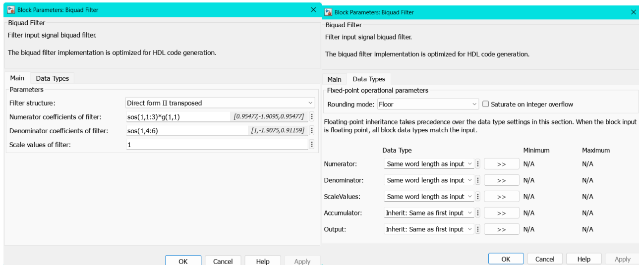
(b) Biquad Filter: Datatypes
