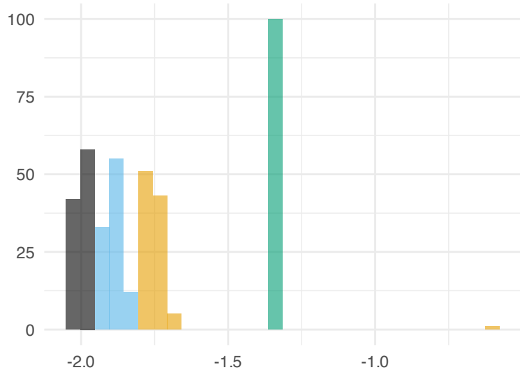
Hydrochem
