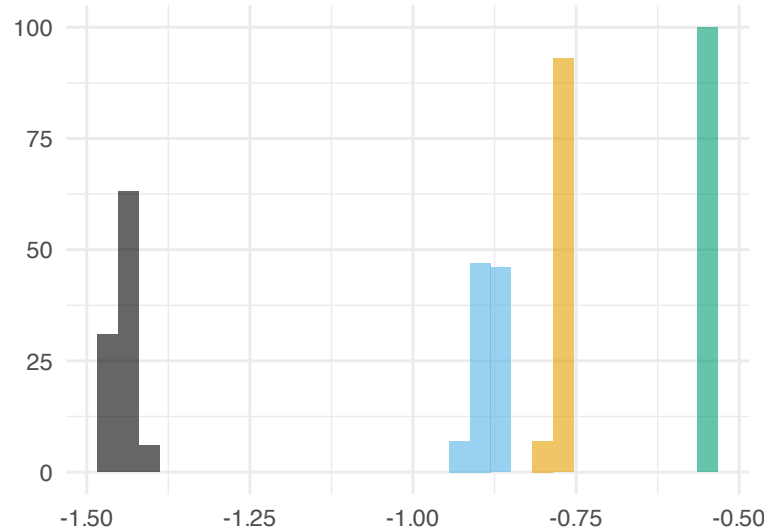
LetterRecognition
