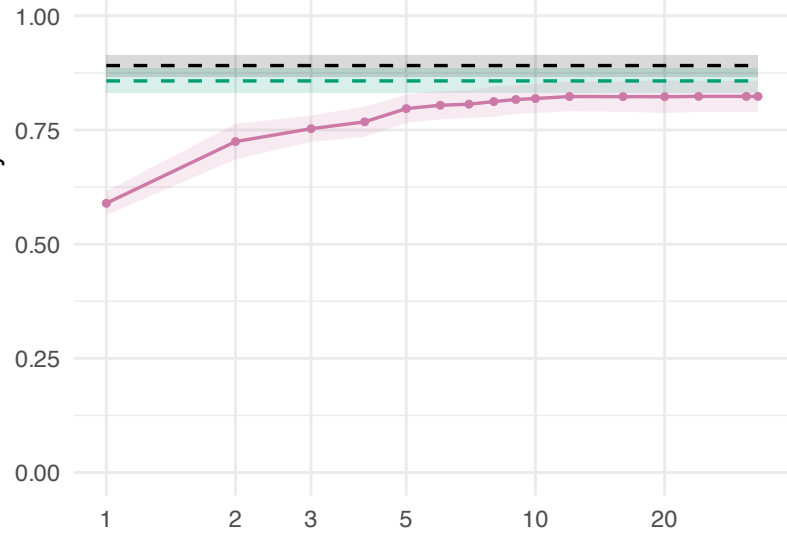
Test accuracy
