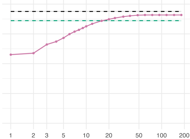
LetterRecognition
