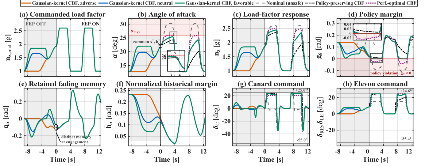
Figure 5: Twin-square benchmark with direct Gaussian history evaluation. The history-aware mechanism persists without relying on the CF one-state exponential realization.
