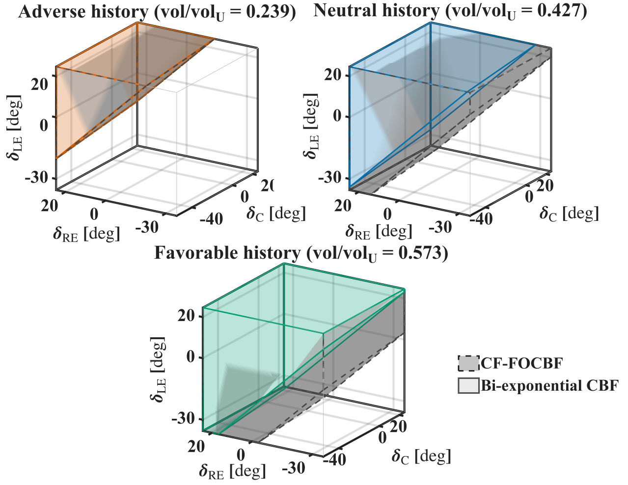
Figure 4: Same-state admissible authority for the bi-exponential kernel. The normalized volumes are 0.239, 0.427, and 0.573 for adverse, neutral, and favorable histories, respectively. The dashed geometry shows the history-matched CF reference.
