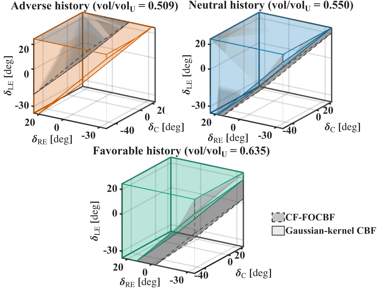
Figure 6: Same-state admissible authority for the Gaussian kernel. The normalized volumes are 0.509, 0.550, and 0.635 for adverse, neutral, and favorable histories, respectively. The dashed geometry shows the history-matched CF reference.
