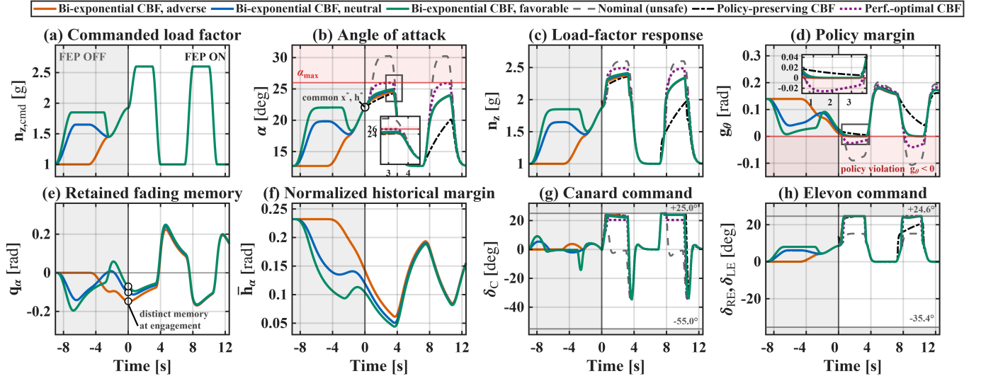
Figure 3: Twin-square benchmark with the bi-exponential kernel. The three preparations reach the common activation condition with different retained memory, producing distinct history-aware policy margins and control responses.
