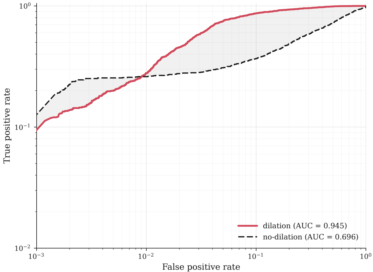
ROC curves: test on SILIVRI2019
