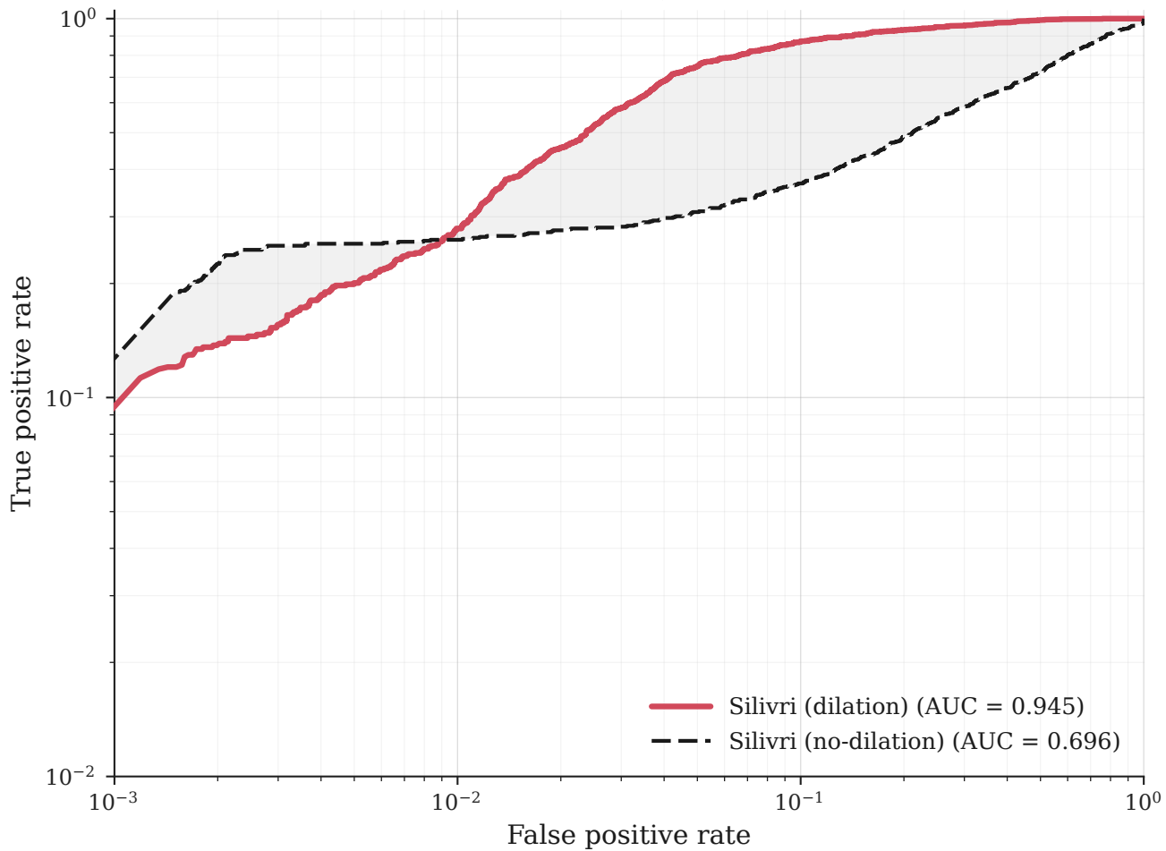
Silivri dilation vs. no-dilation, tested on SILIVRI2019
