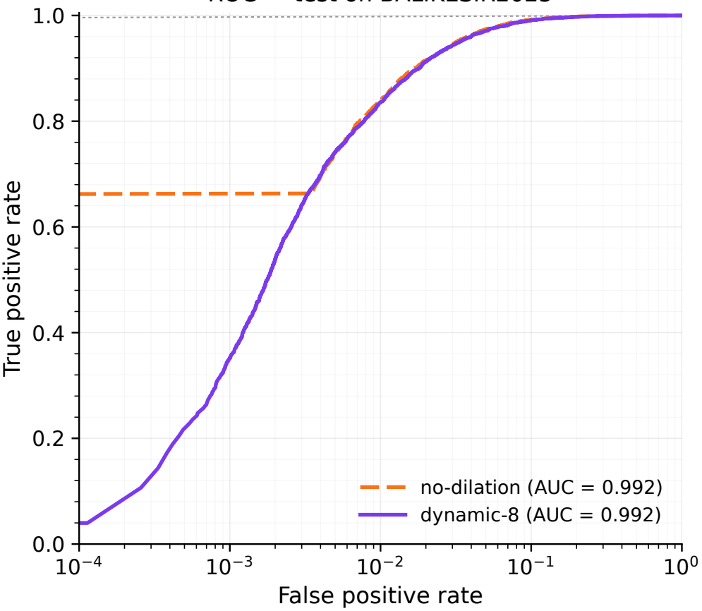
ROC — test on BALIKESIR2025
