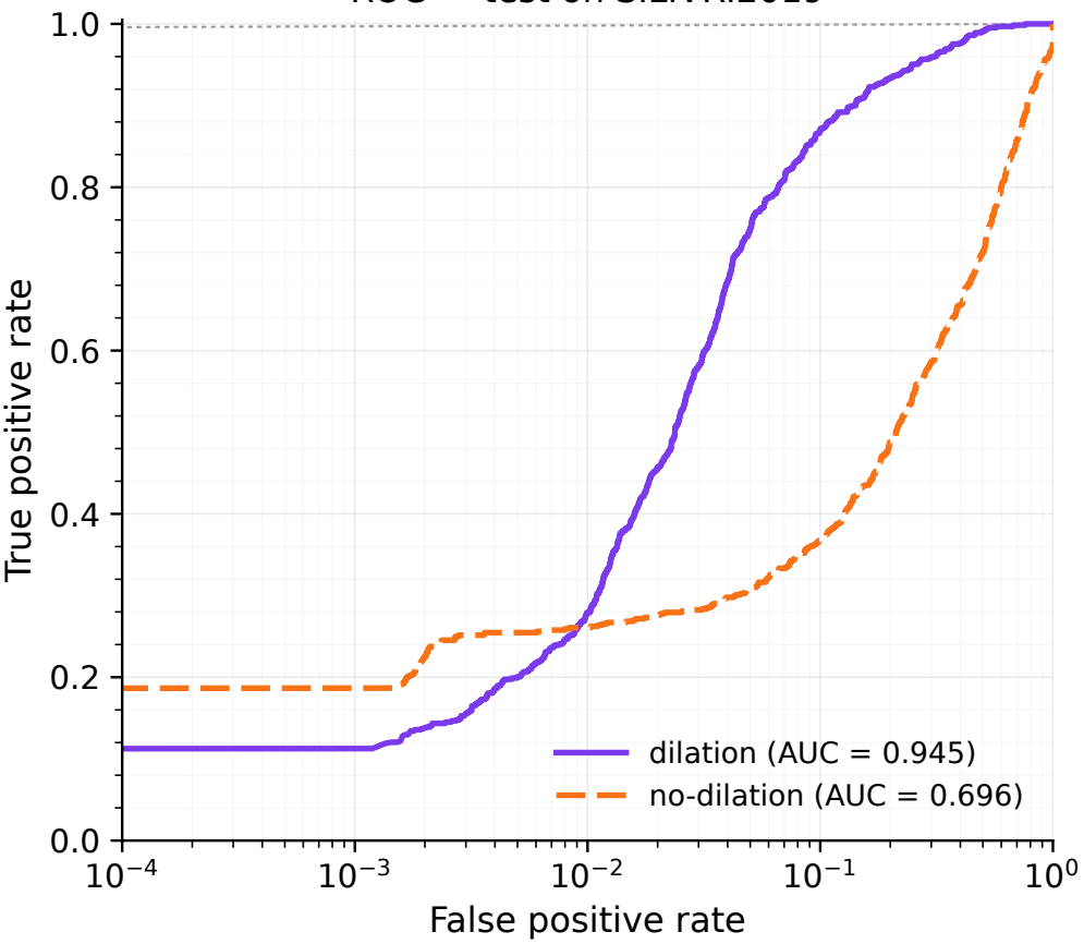
ROC — test on SILVRI2019
