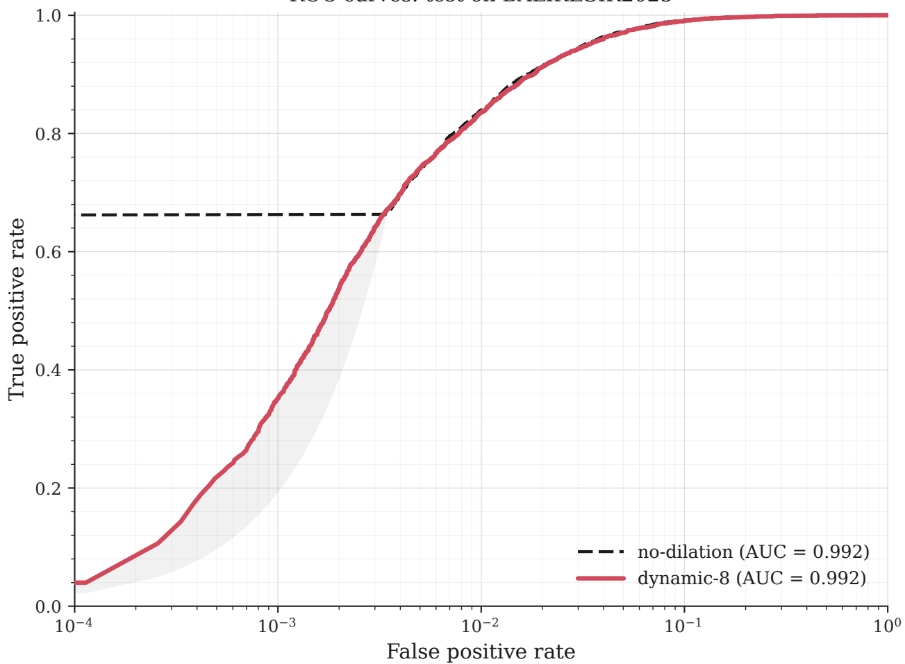
ROC curves: test on BALIKESIR2025
