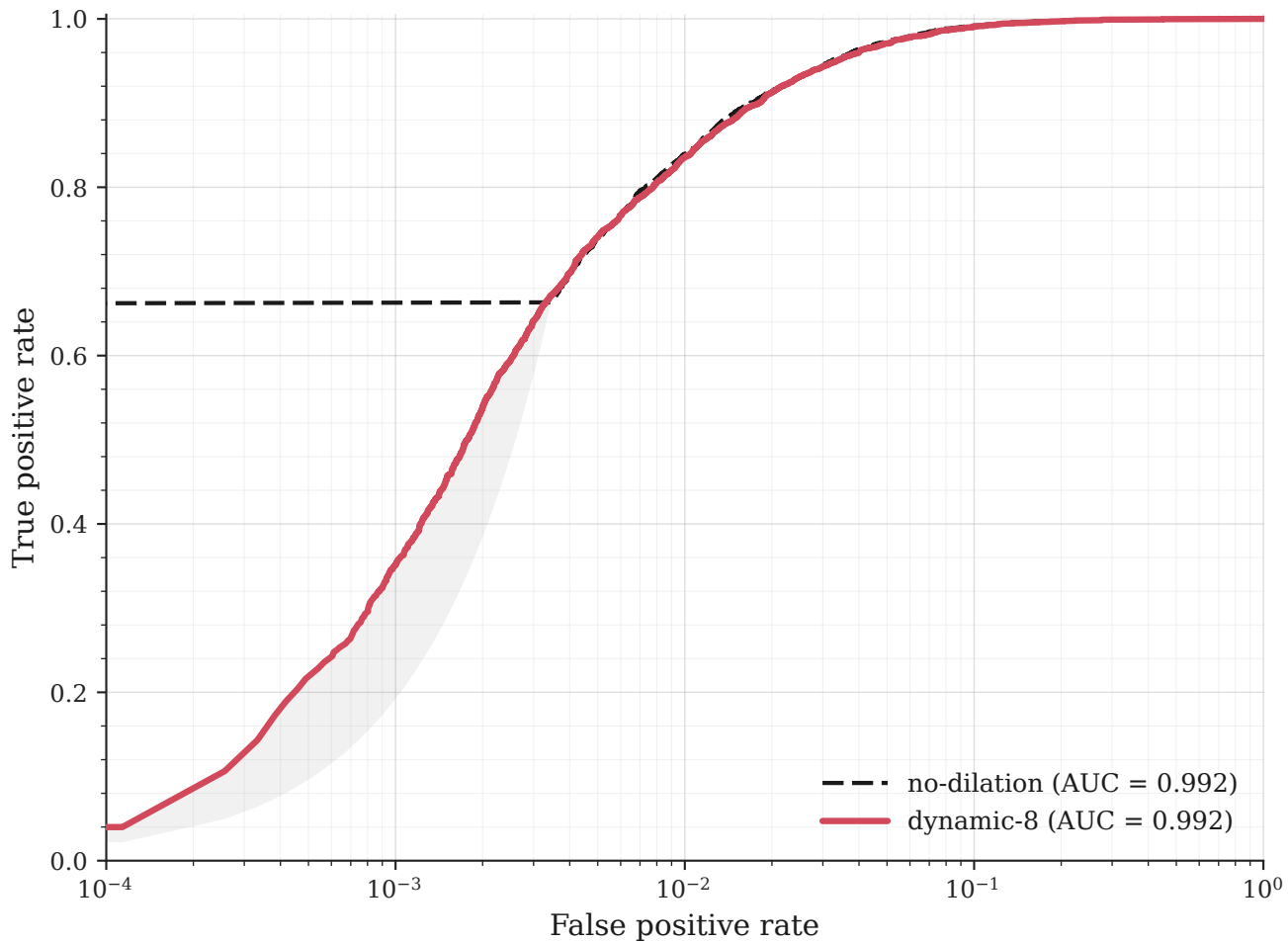
ROC — test on BALIKESIR2025
