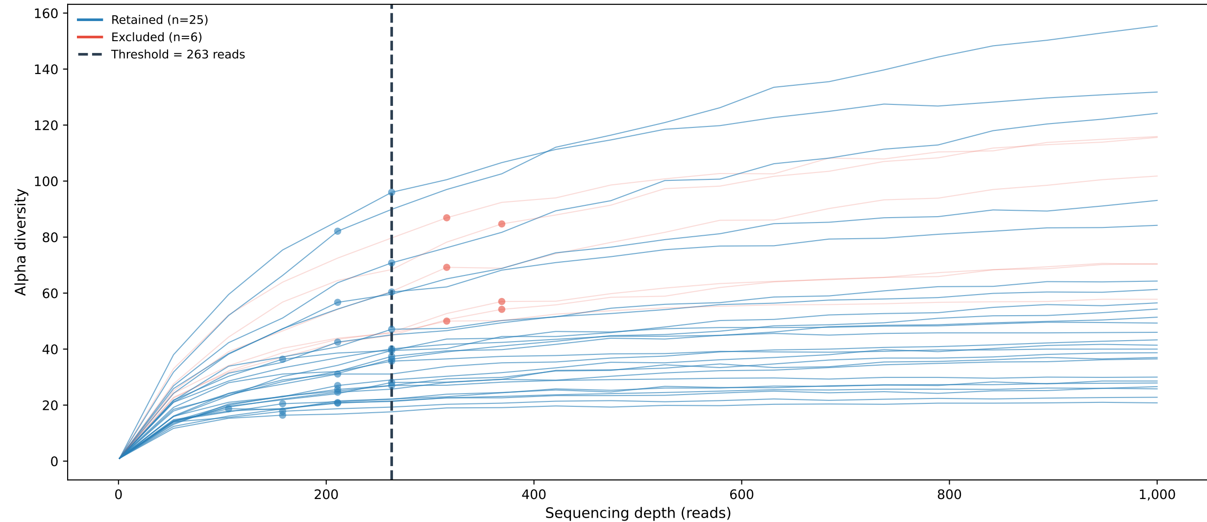
Rarefaction curves (dot = per-sample plateau, dashed = global threshold)
